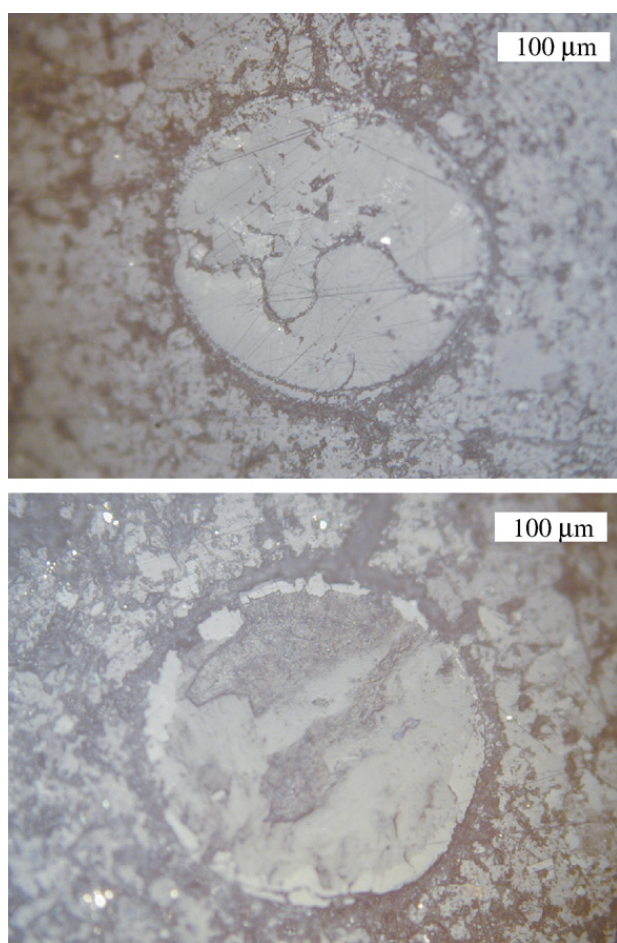
Fig. 2. Reflected light photomicrographs showing well-preserved lycopphyte megaspores in petrographic thin sections of Triassic septaria from the Vanoise massif. In the upper photomicrograph, the megaspore is filled with calcite, while in the lower one, it is filled with phengite.
