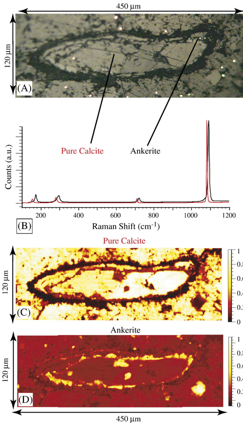
Fig. 8. Raman characterization of carbonates associated with a megaspore within the septaria. A. Optical photomicrograph showing a lycopyle megaspore from the same septaria in which the megaspores depicted in Fig. 2 were found. B. Raman spectra of the minerals present in the central part of the spore and beneath the spore cell wall, respectively, pure calcite (red spectrum; vibrational bands at 155, 280, 710 and 1085 cm -1 ) and ankerite (black spectrum; this spectrum shows a shift to higher frequencies of about 15 cm -1 compared to the calcite reference spectrum). C. and D. Raman mapping showing the correlation index of each spectrum with the reference spectrum of pure calcite (C) and ankerite (D), respectively (mosaics compiled from ~40,000 Raman spectra). Higher index values indicate a greater correlation between the sampled spot and the reference. Calcite thus appears as yellow/white in C. and ankerite appears as yellow/white in D.
